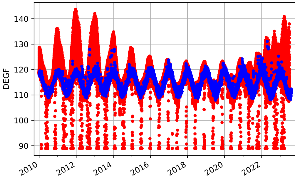
Solar array temps at off-nominal roll 5 - 10 degrees
